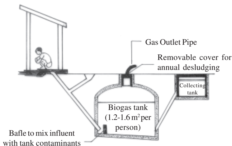
Fig. 30.2: Biogas Plant
