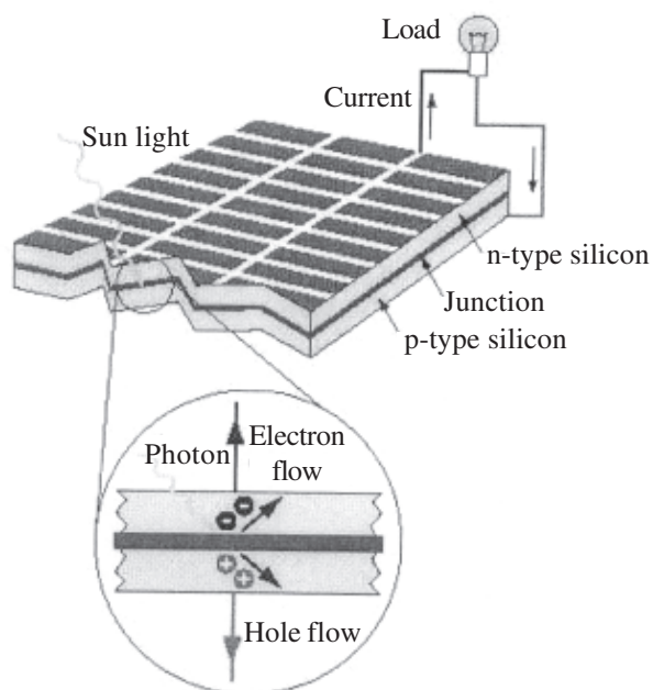
Fig. 29.3: Photovoltaic cell
